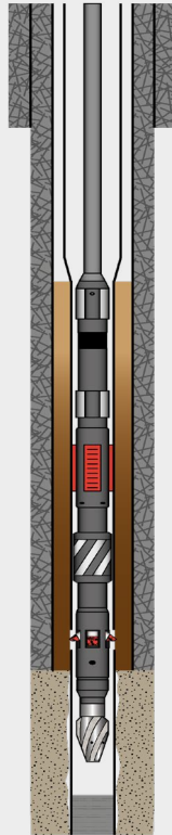
2. Make cut & verify free
