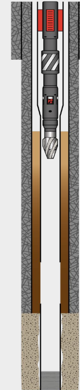
6. Relocate & Pull Casing
