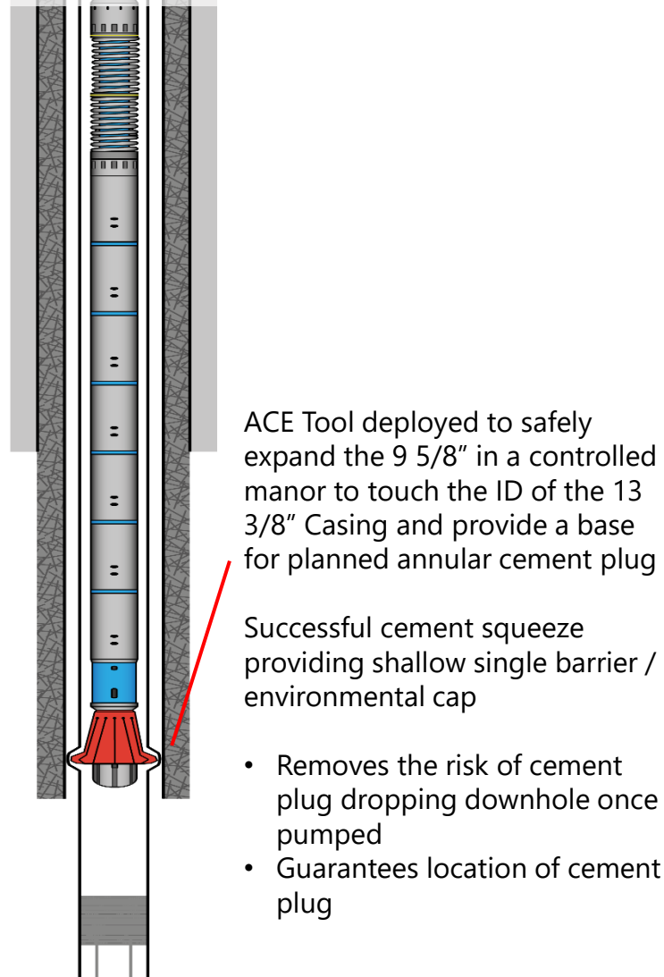
ACE Tool Operation
