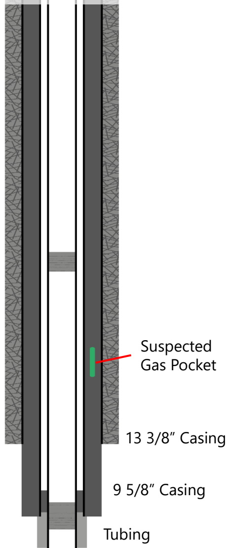
Current Well Status
